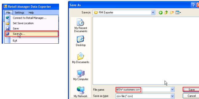
Figure 7 Save Dialog
